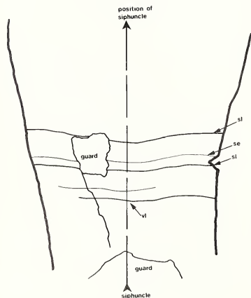
TEXT-FIG. 9. Camera-lucida drawing of the suture lines and septal lines exposed on the ventral side of the oral third of the holotype of Payloviteuthis cantiana (Spath, 1939), C.37844, \times 25 . The reproduced lines are those visible in the seventh and eighth camerae from the oral end of the specimen in Pl. 22, fig. 1G. vl—ventral lobe. Other abbreviations as in text-fig. 7.
